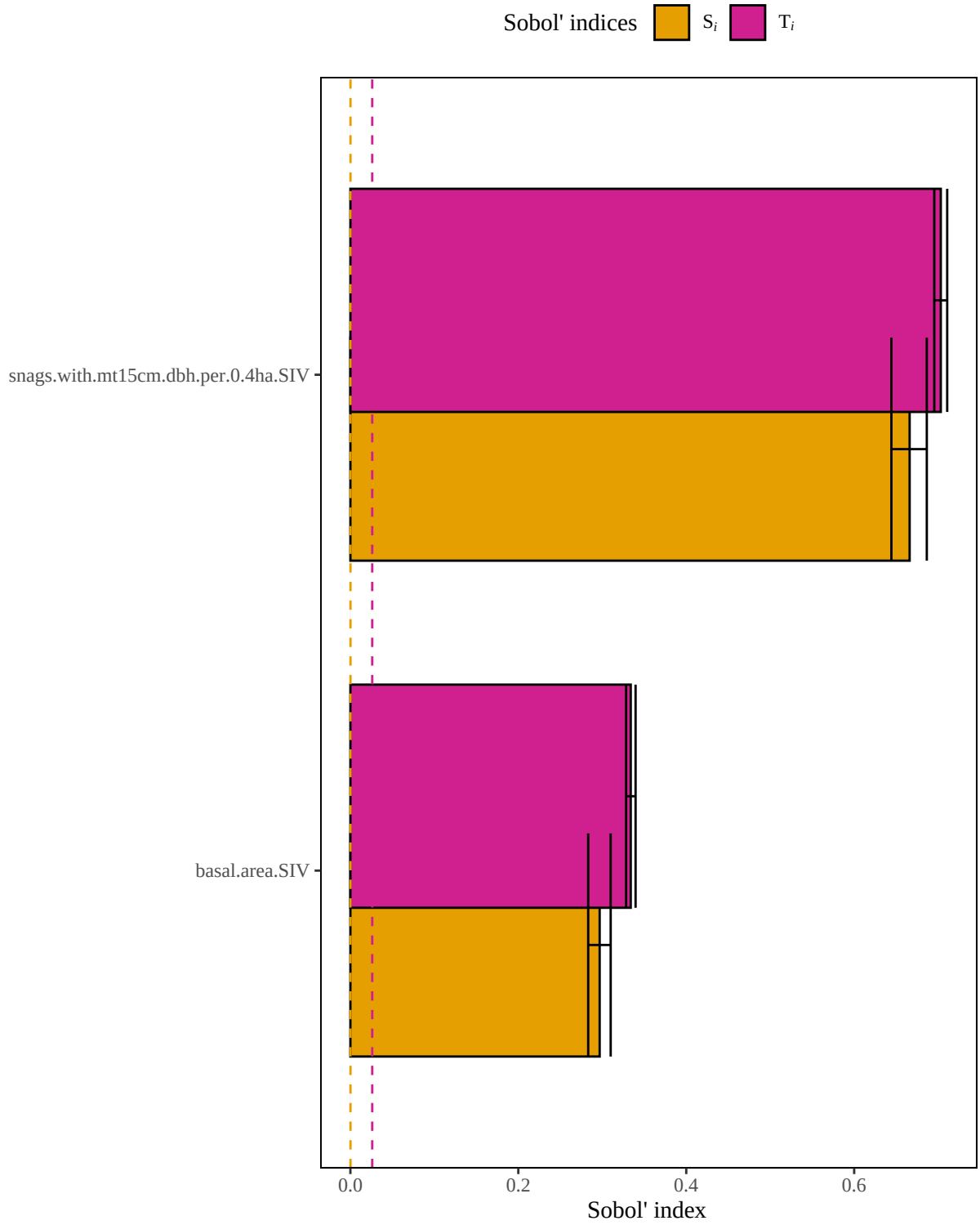
Figure 5. Results of a sensitivity analysis for the downywoodpecker model based on a geometric mean structure. Dashed lines represent baseline numerical approximation error for S_i and T_i ( i.e. , dummy variables).
